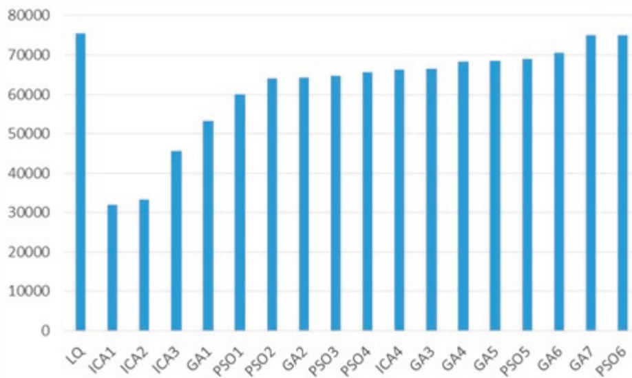
Fig. 7. Volume of earthworks at different methods (M3)
