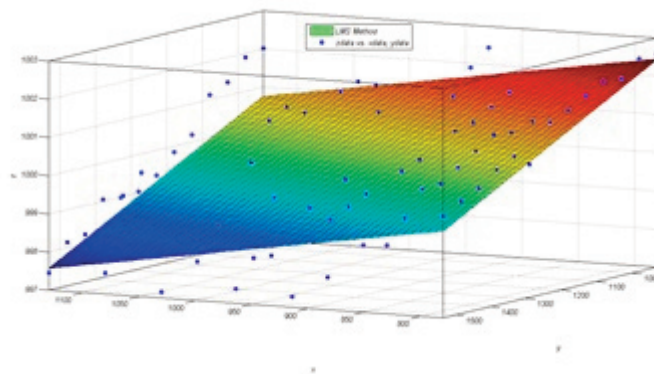
Fig.5. Estimating Leveling Surface by ICA
