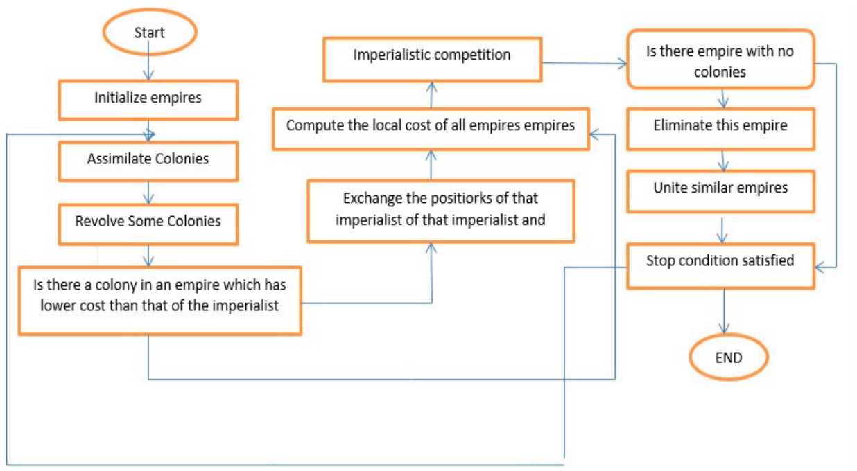
Fig.4. Flowchart of the imperialist competitive algorithm
