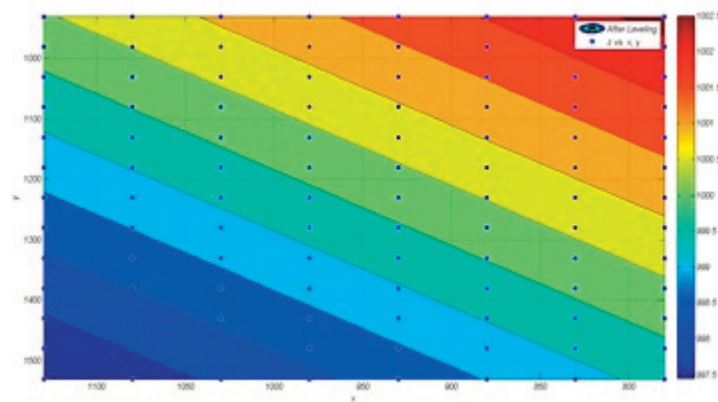
Fig. 6. Map leveling of ground at different levels by ICA
