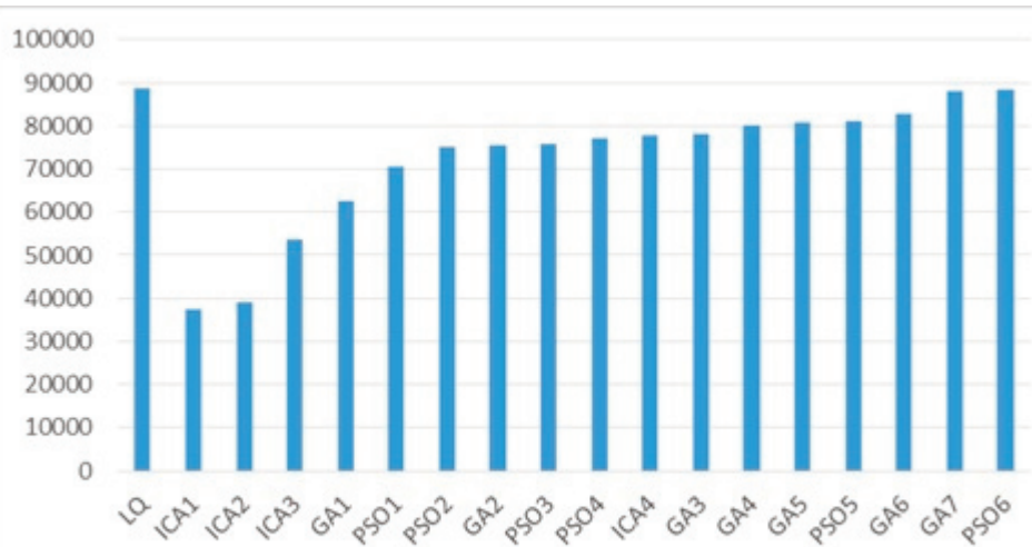
Fig.10. Percentage of decrease in total consumption energy ratio for different models (MJ)
