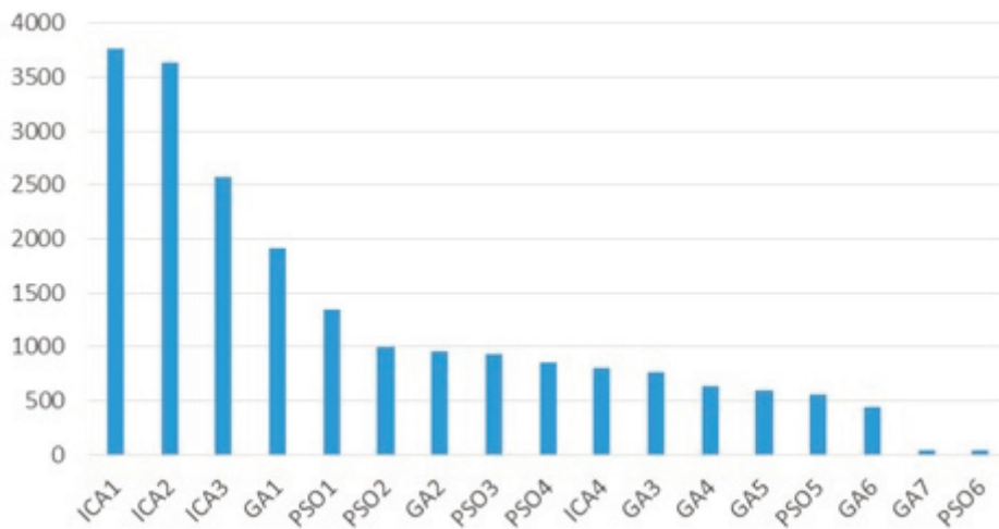
Fig. 8. Cost saving in energy consumption for different models (Thousand Rials)
