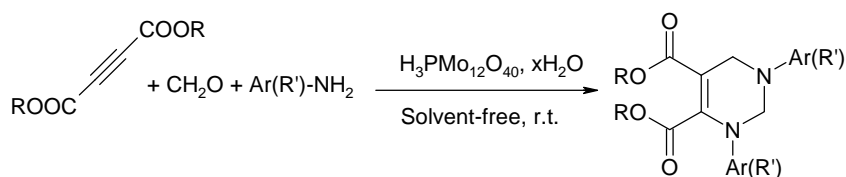
Scheme 1. Preparation of tetrahydropyrimidine derivatives in the presence of \text{H}_3\text{PMo}_{12}\text{O}_{40} .
