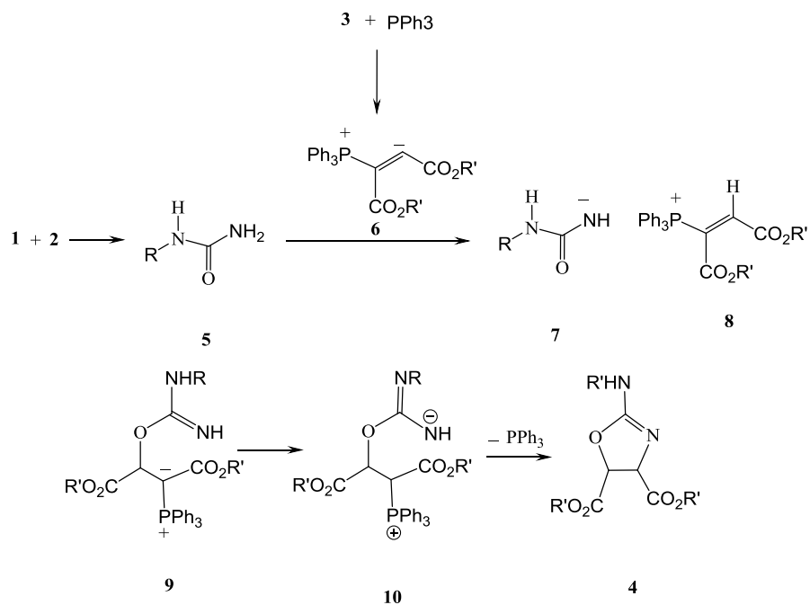
Scheme 2: Proposed mechanism for the formation of 4 .
