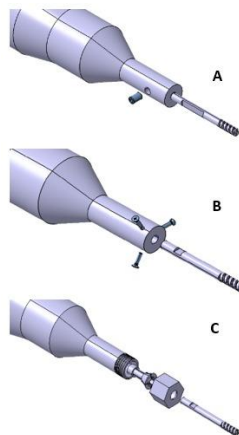
Figure 3. Connection mechanism of cutting tool by using A) a screw B) three screw C) cone collet
