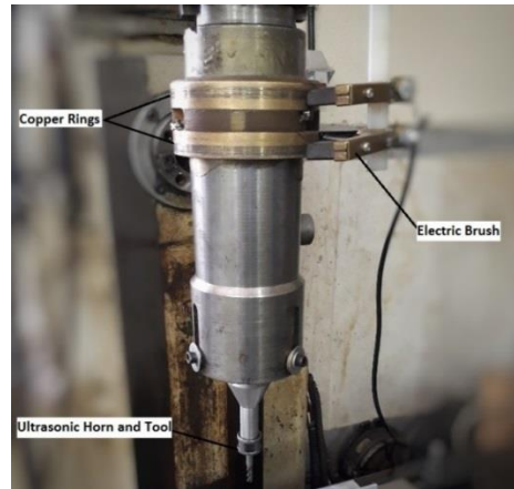
Figure 7. Ultrasonic Vibration assisted end milling
