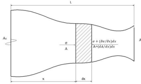
Figure 1. A vibratory rod with a random cross-section
