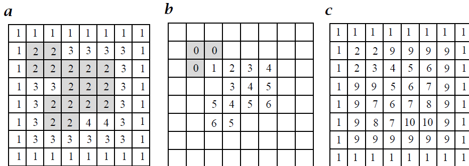
Figure 4. Lower complete transformation: a) original gray image; b) geodesic function and c) lower complete image.
