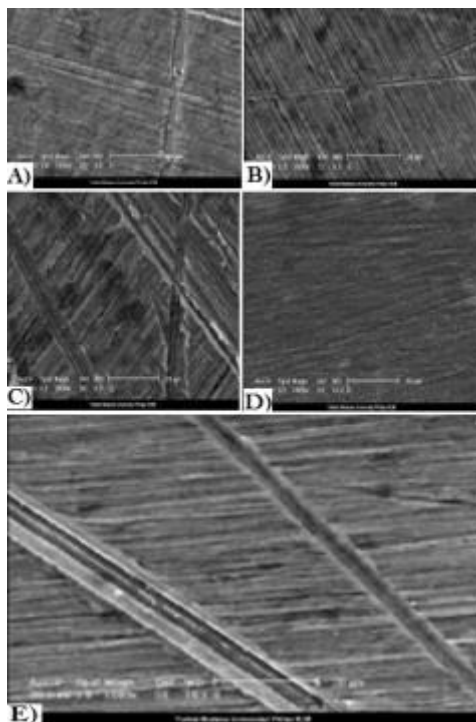
Figure6. The SEM images from the surface of Vt20 in different conditions: A) pH=2, T=25 °C, B) pH=3, T=25 °C, C) pH=2, T=40 °C, D) pH=3, T=40 °C, E) Culture: pH=2, T=25 °C
