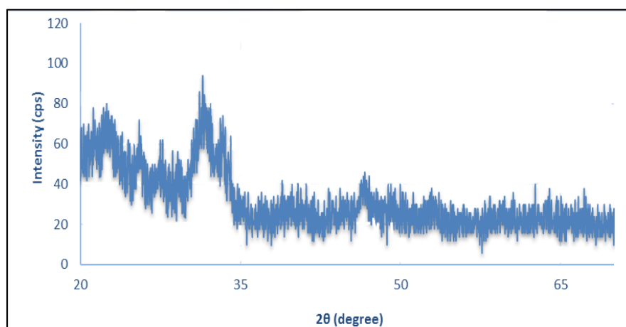
Fig. 1. X-ray diffraction pattern of synthesis of S53P4 bioglass nanopowder
