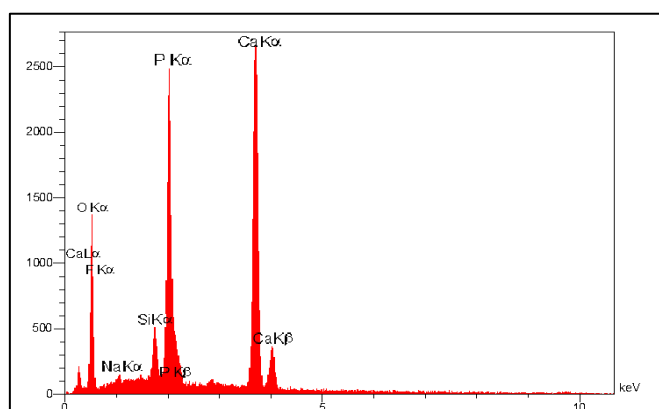
Fig. 16. EDS analysis of BG-FA nanocomposites
