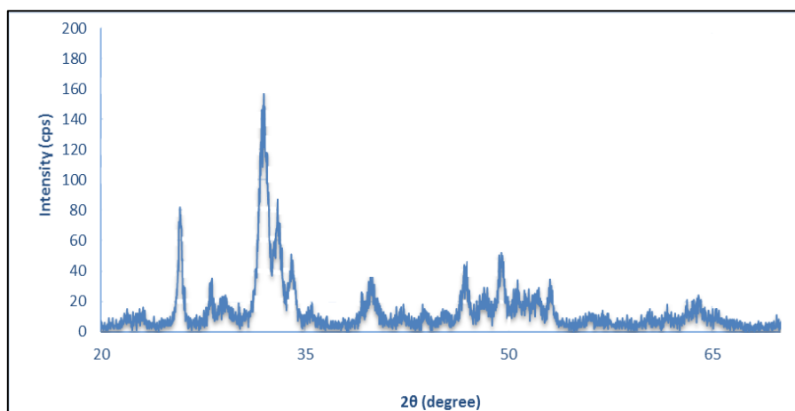
Fig. 2. X-ray diffraction pattern of fluorapatite nanoscale
