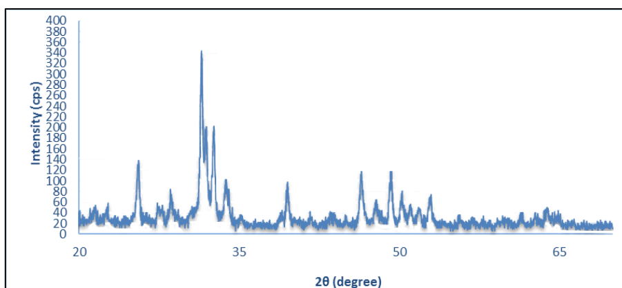
Fig. 5. X-ray diffraction pattern of 30% S53P4 BG-FA nanocomposite
