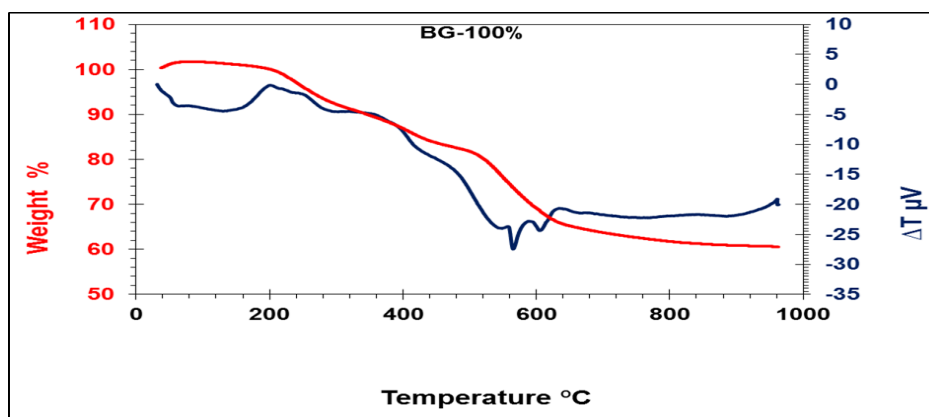
Fig. 6. STA analysis of S53P4 bioglass
