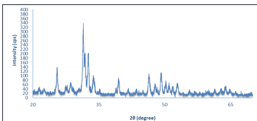
Fig. 4. X-ray diffraction pattern of 20% S53P4 BG-FA nanocomposite
