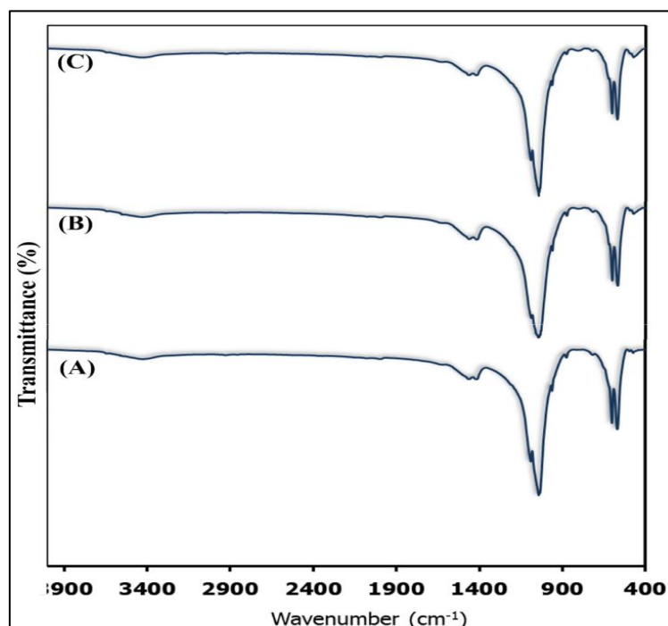
Fig. 9. Infrared spectroscopy analysis of FA-S53P4 BG nanocomposite, A) 10%, B) 20%, C) 30%.
