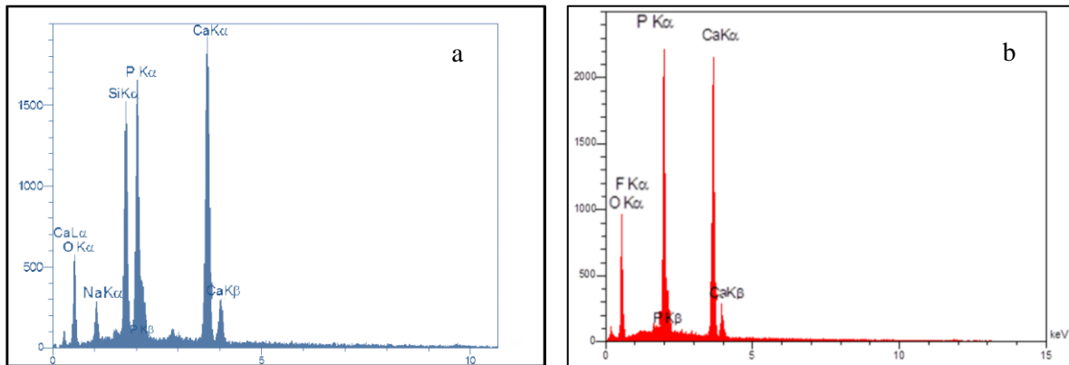
Fig. 14. EDS Analysis of a) S53P4 bioglass, b) fluorapatite nanopowders
