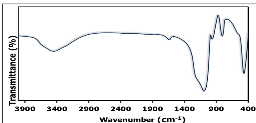
Fig. 7. Infrared spectroscopy analysis of S53P4 bioglass
