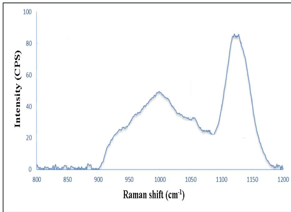
Fig. 10. S53P4 bioglass spectroscopy test
