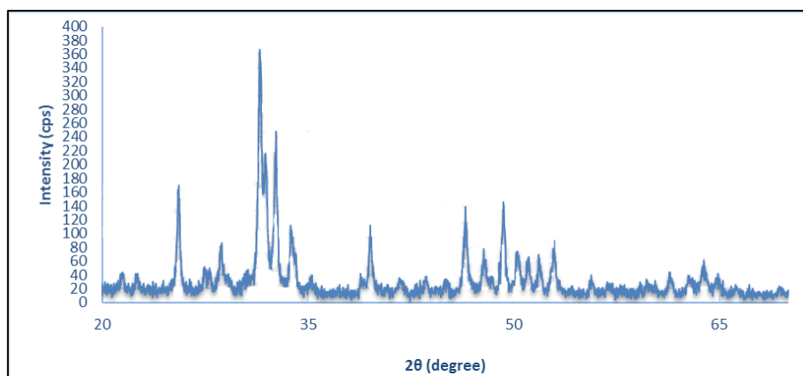
Fig. 3. X-ray diffraction pattern of 10% S53P4 BG-FA nanocomposite
