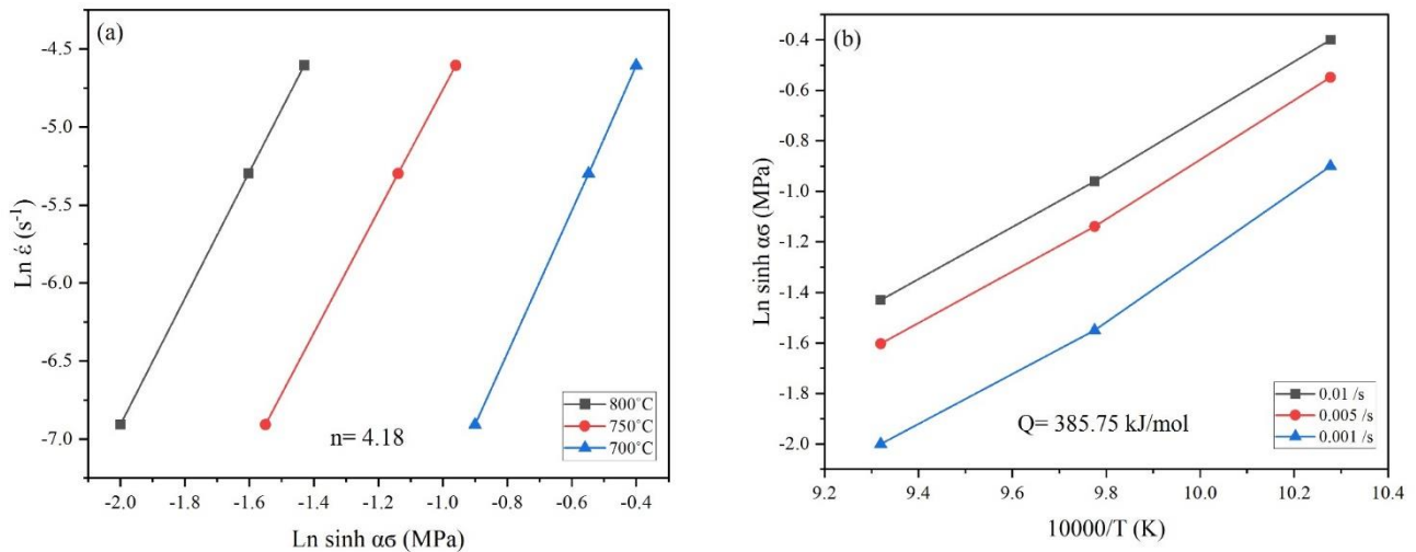
Fig. 11. The plot of (a) \ln \dot{\epsilon} versus \ln \sinh (\alpha \sigma) at different temperatures and (b) the \ln \sinh (\alpha \sigma) data as a function of inverse temperature at various strain rates.
