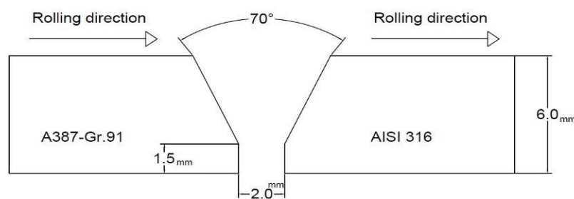
Fig. 1. Schematic of the joint design.
