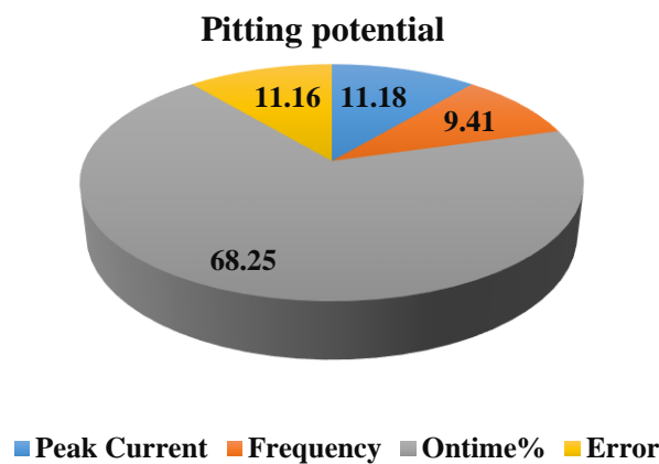
Fig. 6. Influence of PCGTAW process parameters on pitting potential of weld metal and error obtained from pooled ANOVA.
