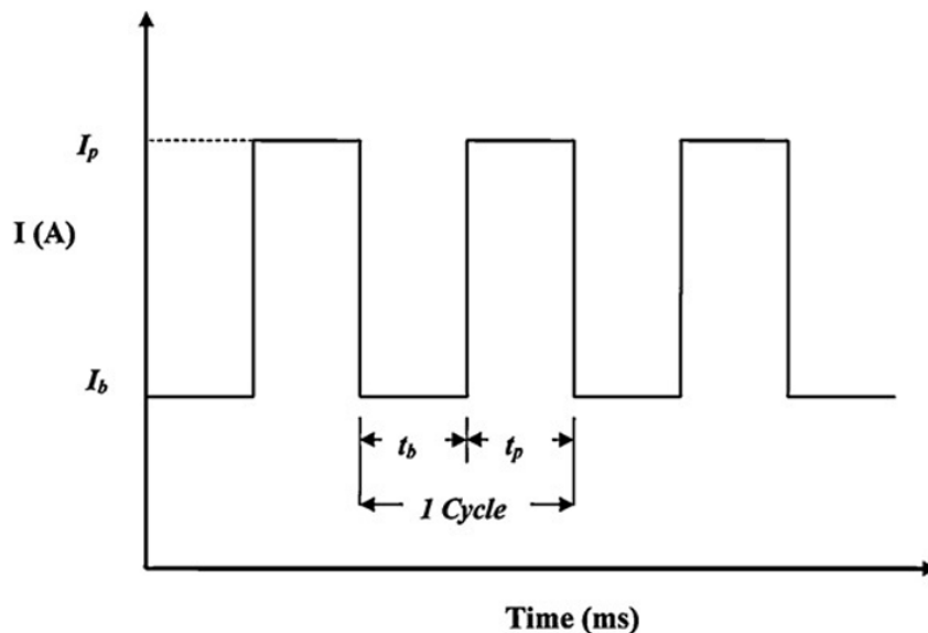
Fig. 2. Current-time chart. I_p is the peak current (A), I_b is the background current (A), t_p is the peak current duration (ms), and t_b is the background current duration (ms) [12].
