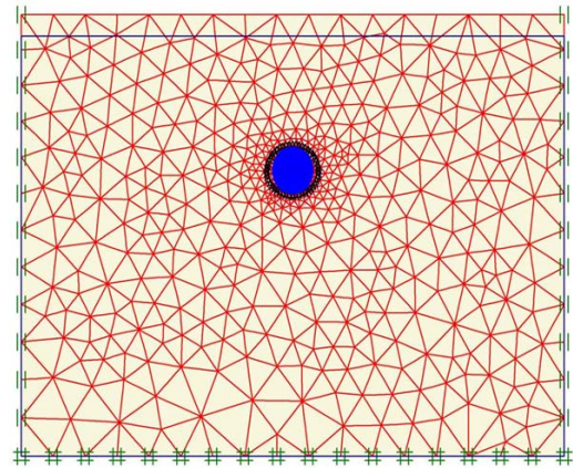
Fig. 11. Deformed mesh due to the ground strength reduction Extreme Total displacement 187.96 \cdot 10^{-3} m
