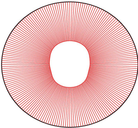
Fig. 14. Axial force diagram in tunnel lining after lowering the ground water table. Extreme Axial force -977.12kN/m
