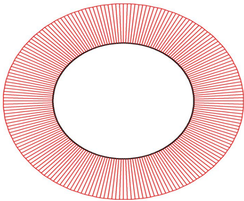
Fig. 9. Displacements of tunnel lining under internal pressure Total displacement (Utot).Extreme Utot 2.34 \cdot 10^{-3} m
