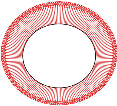
Fig. 9. Displacements of tunnel lining under internal pressure Total displacement (Utot).Extreme Utot 2.34 \cdot 10^{-3} m
