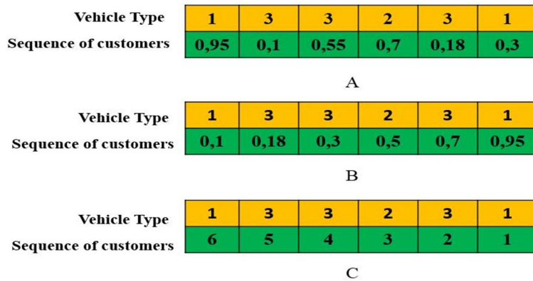
Fig 1-A. The proposed two-string chromosome before sorting the randomly generated the numbers in the second string Fig 1-B. The proposed two-string chromosome after sorting the randomly generated the numbers in the second string Fig 1-C. Proposed two-string chromosome with the sequenced customers
