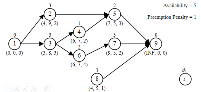
Figure 1. Problem instance for the PRCPSPWETPP
