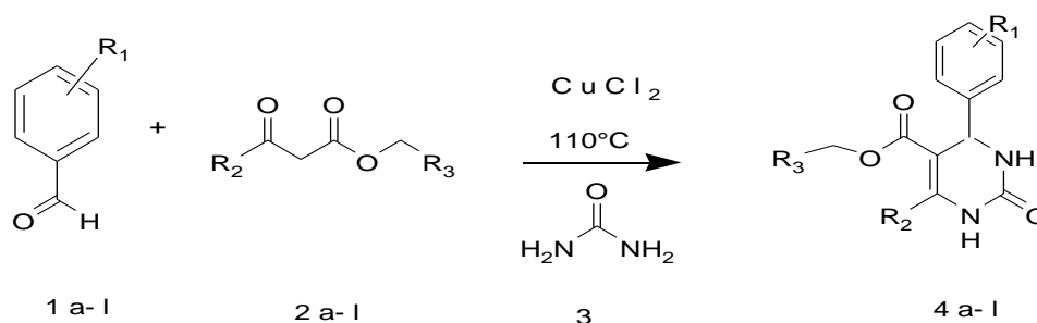
Scheme 1. Biginelli type reaction for synthesis of dihydropyrimidone derivatives
