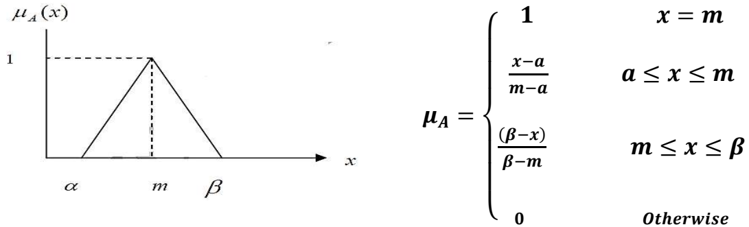
Fig. 2: Triangular Numbers
