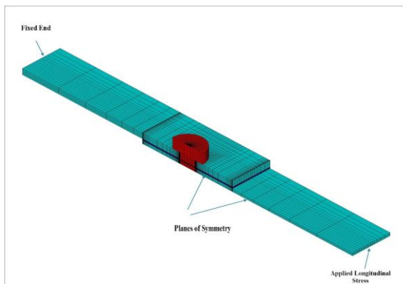
Fig.8 Applied loads and boundary conditions in three dimensional finite element model.
