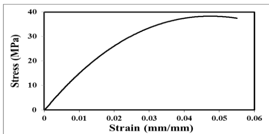
Fig.4 Engineering stress-strain curve of Loctite 3421 adhesive.
