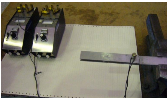
Fig.7 Measuring clamping force with load cell.
