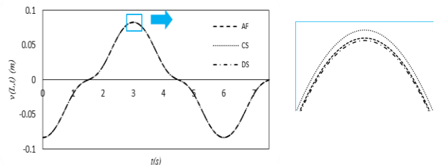
Fig.13 Response of the drag force for all three foundation models DS, AF and CS by taking into account the three first Fourier's series terms.
