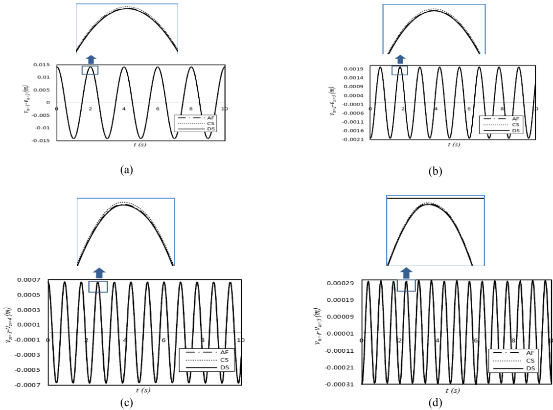
Fig. 12 Variation of results in employing the number of Fourier's series terms, a) Difference between employing 2 terms and 1 term, b) Difference between 3 included terms and 2 terms, c) Difference between 4 and 3 considered terms d) Difference between 5 and 4 included terms.
