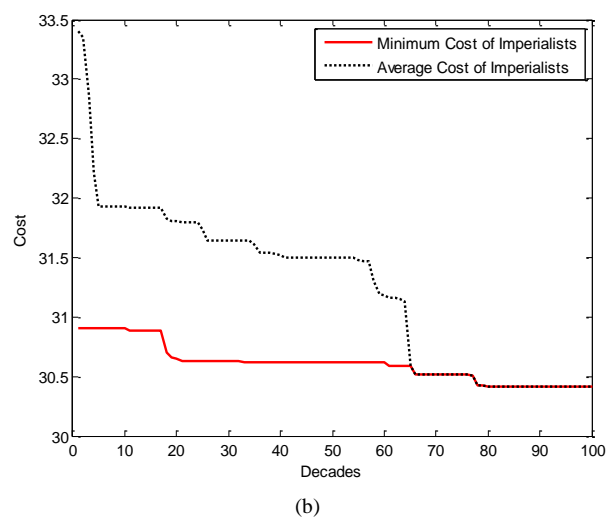
Fig. 4 Convergence of the objective of minimum weld area, (a): EBW, (b): SAW
