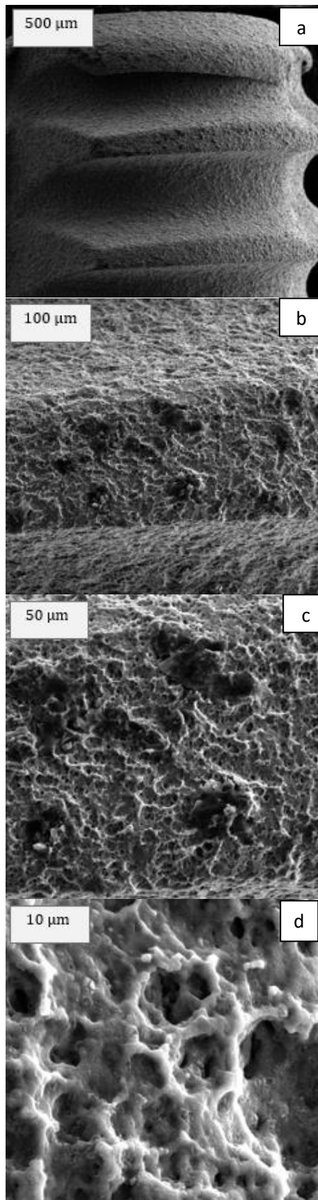
Fig. 3. SEM images related to SLActive surface treatment method for 3A titanium implant fixture.
