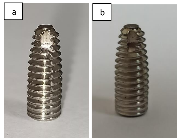
Fig. 1. Implant fixture 3A a) before and b) after sandblasting operation and acid etching.
