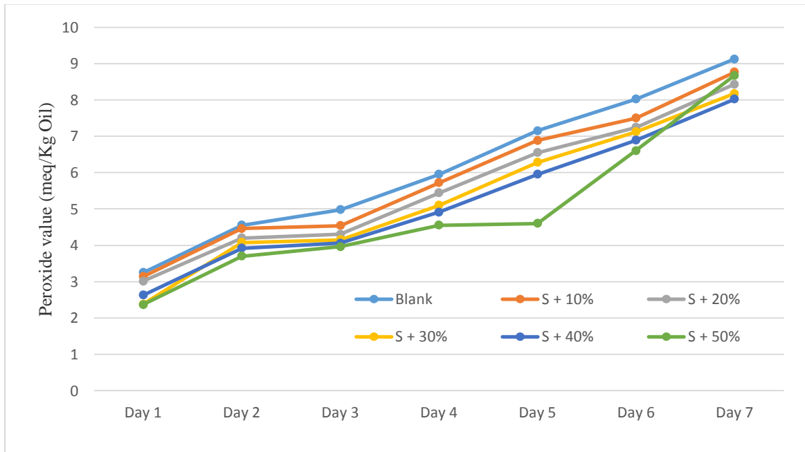
Figure 2 - Peroxide value of soybean oils containing 10-50% of ostrich fat, during 7 days storage in the oven (meq/Kg oil)
