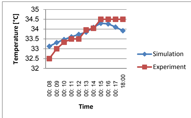
Fig.13: Comparison of measured results and computer simulation results in 2013/7/21 (five-door section)
