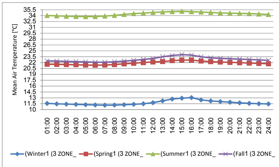
Fig.8: The thermal behavior comparison of three-door section in northeast orientation in the first day of different seasons
