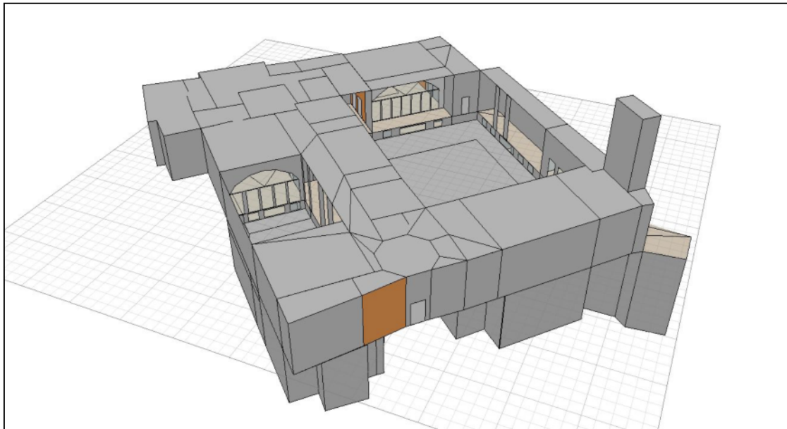
Fig.5: The building (Rasoulia home) model reconstructed in Ecotect
