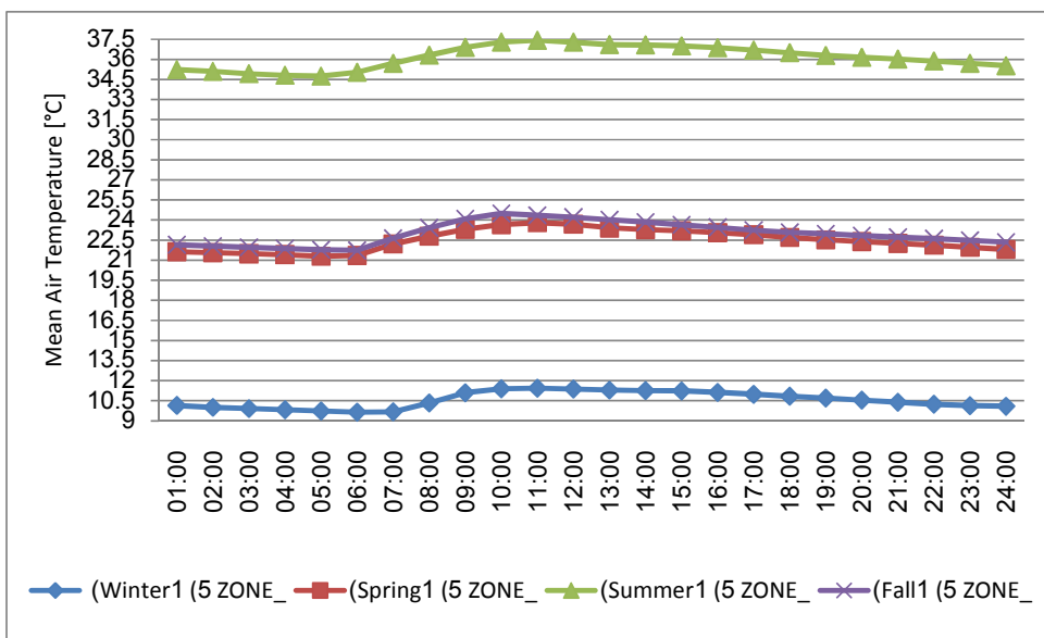
Fig.10: The thermal behavior comparison of three-door section in northwest orientation in the first day of different seasons
