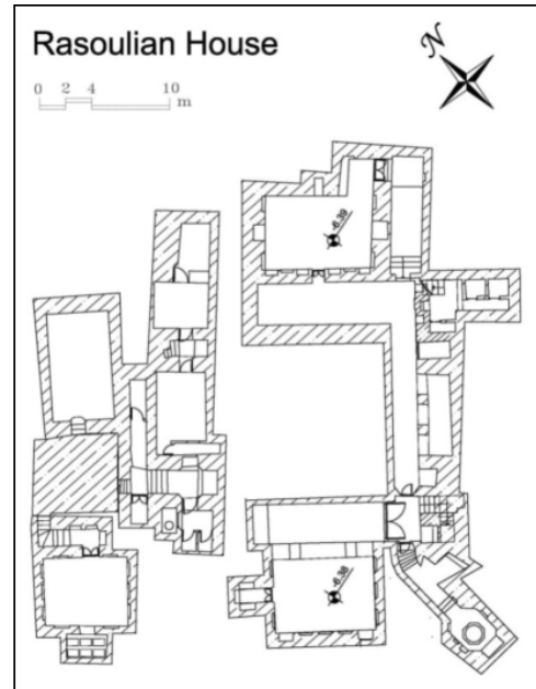
Fig.4: The basement of Rasoulia home
