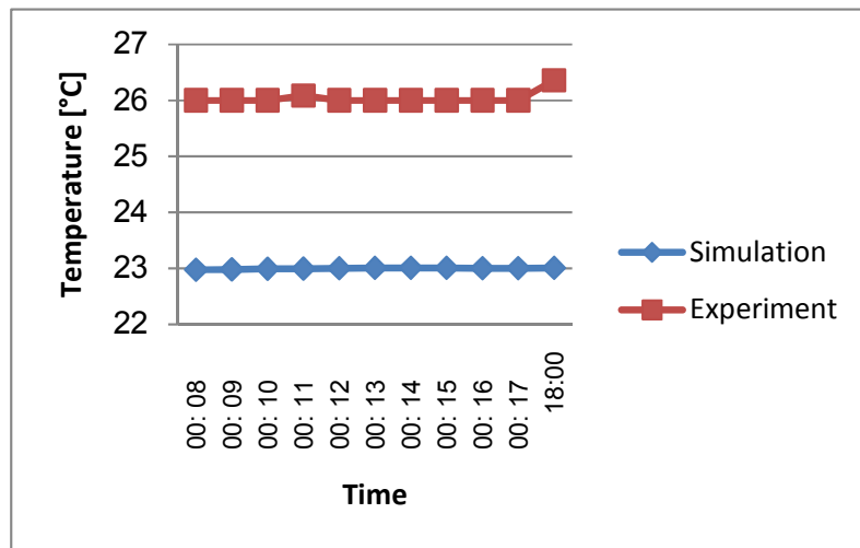
Fig.16: Comparison of measured results and computer simulation results in 2013/7/21 (cellar section)
