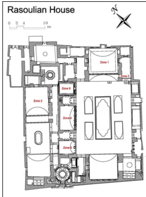
Fig.3: The first floor of Rasoulia home
