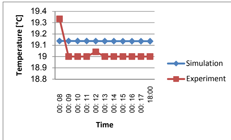
Fig.15: Comparison of measured results and computer simulation results in 2013/7/21 (coastal section)
