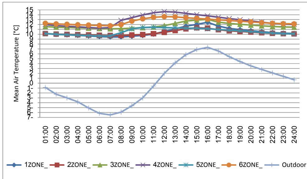
Fig.12: The thermal behavior of winter sections in the first day of winter
