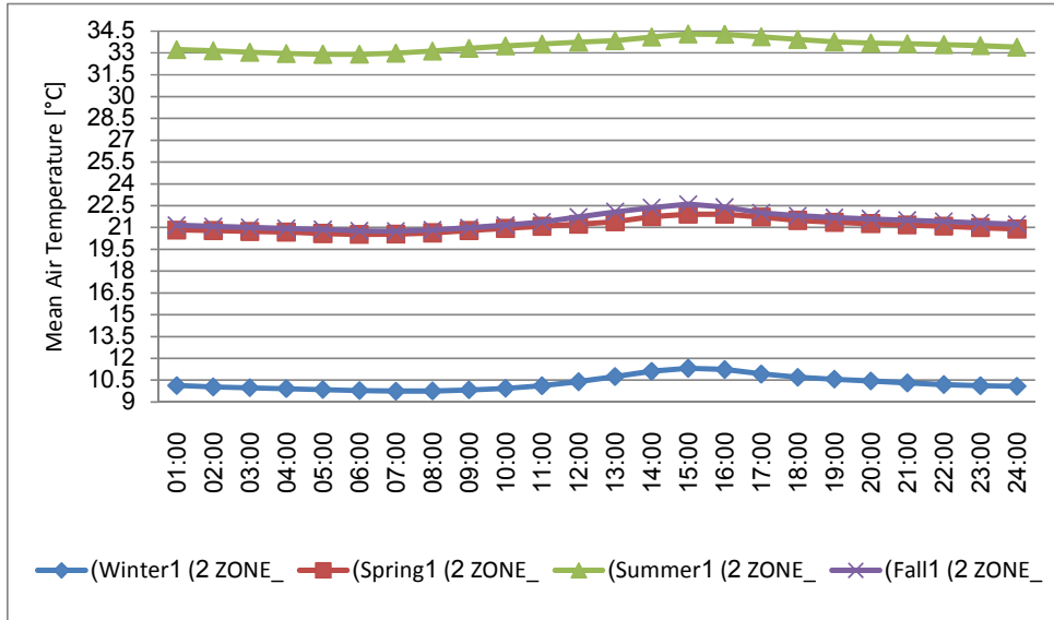
Fig.7: The thermal behavior comparison of five-door section in northeast orientation in the first day of different seasons
