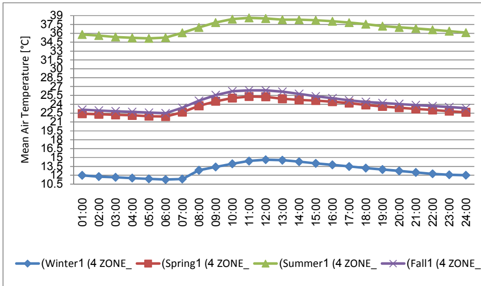
Fig.9: The thermal behavior comparison of five-door section in northwest orientation in the first day of different seasons
