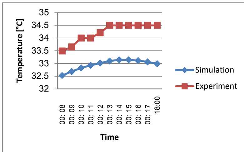
Fig.14: Comparison of measured results and computer simulation results in 2013/7/21 (wind tower section)
