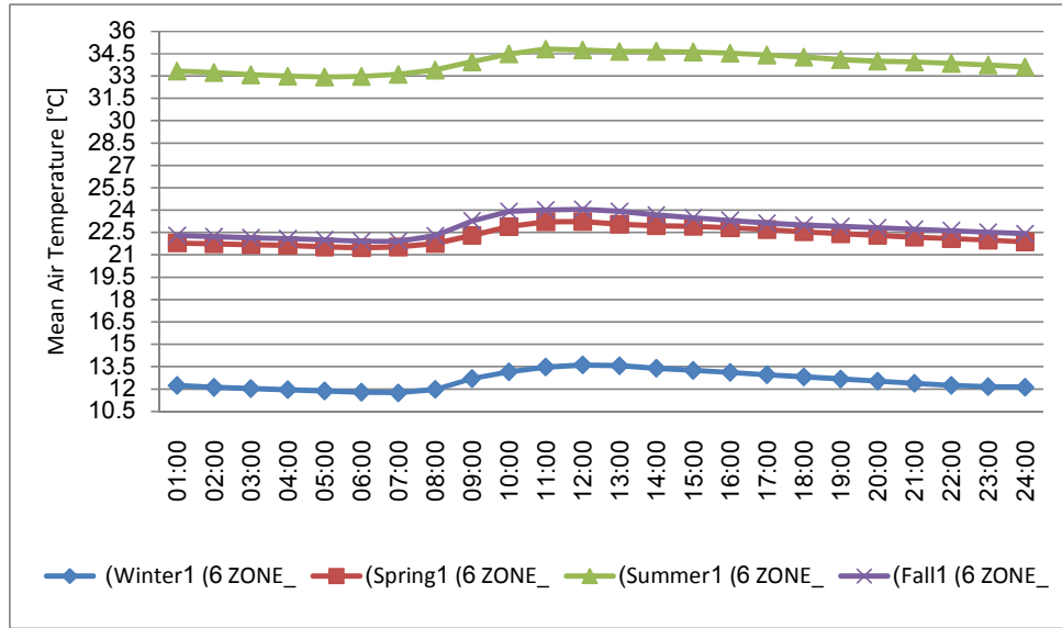
Fig.11: The thermal behavior comparison of three-door section in northwest orientation in the first day of different seasons
