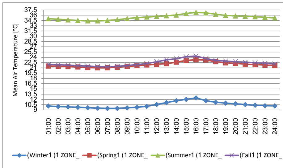
Fig.6: The thermal behavior comparison of seven-door section in northeast orientation in the first day of different seasons
