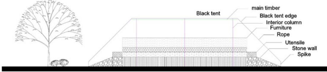
Fig. 9: Section of a Black Tent and Its Interior Arrangement.
