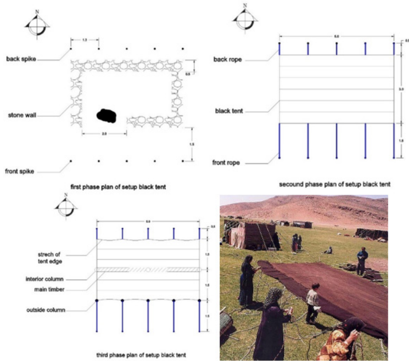
Fig. 14: Installation stages of the black tent in Vorghah
