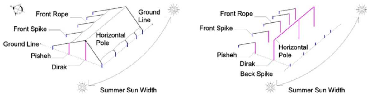
Fig. 17. Arrangement of Dirak, Pisheh, rope, and hooks in front and back of the black tent in summer
