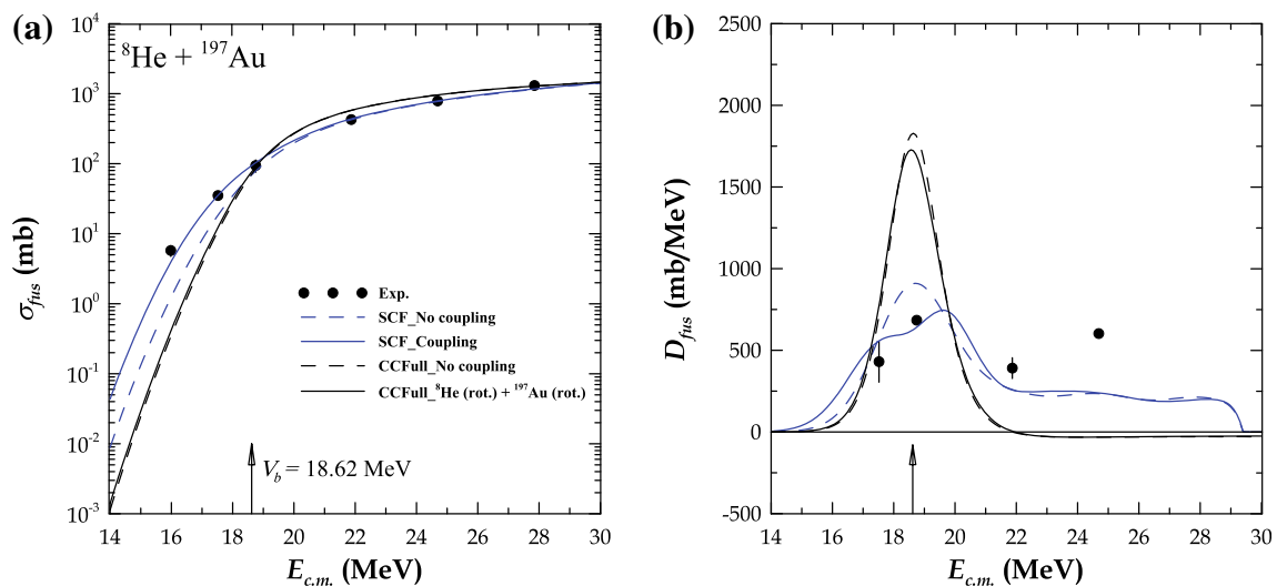
Fig. 2 The comparison of the semiclassical and full quantum mechanical calculations using SCF code (blue curves) and CCFull code (black curves) with the experimental data (black filled circles) [32] for {}^8\text{He} + {}^{197}\text{Au} system. a for the total fusion cross
