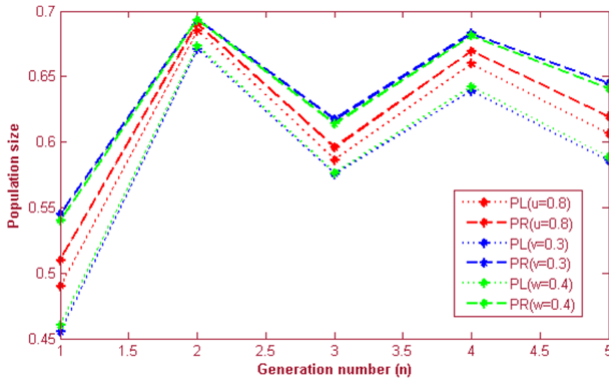
Figure 6: The discrete change-over the population size and the generation number of the System (66) for u = 0.8, v = 0.3 and w = 0.4 .
