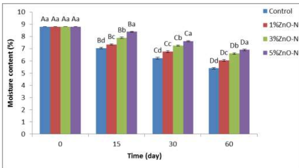
Fig.2. Moisture content of peanuts. Control: peanuts packed with potato starch/CSAE. Different small and capital letters illustrate significant difference among means \pm SD (n=3) of various concentrations of ZnO-N and one specimen during preservation respectively.
