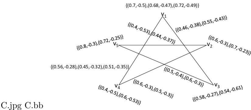
Figure 3: The BVHFG
