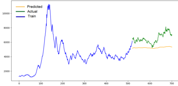
Fig.7. Prediction chart of Shapna stock with sigmoid activation function
