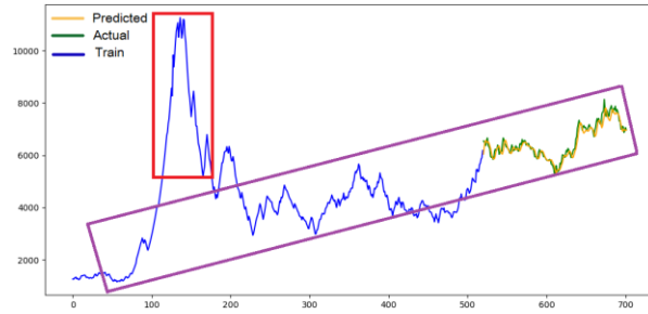
Fig.10. Forecasting Shapna stock with out-of-range data
