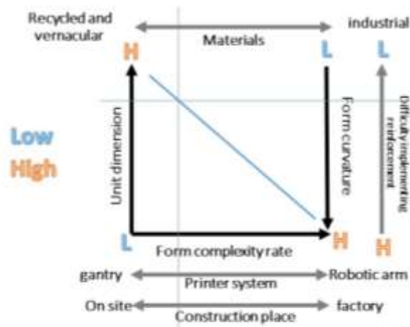
Fig 12. Decision matrix for building housing with 3D printing in different conditions
