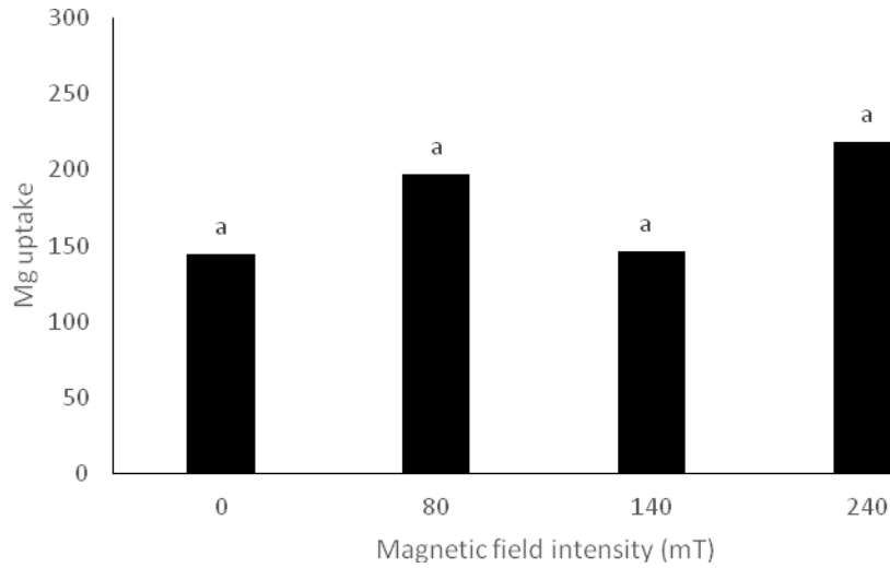
Figure 16. Effect of various magnetic field intensity on plant Mg uptake
