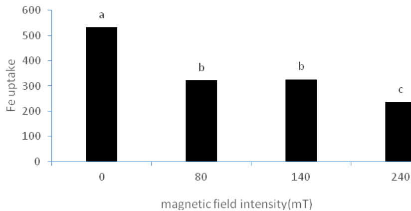
Figure 4. Effect of various magnetic field intensity on plant Fe uptake
