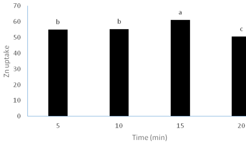
Figure 7. Effect of different time exposure of magnetic field on Zn uptake
