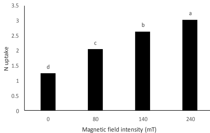
Figure18. Effect of various magnetic field intensity on plant N uptake
