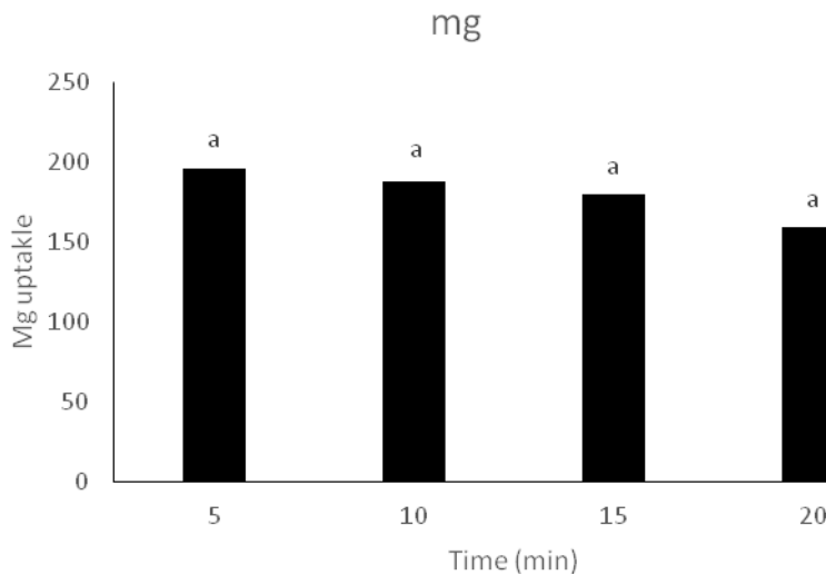
Figure 17. Effect of different time exposure of magnetic field on Mg uptake
