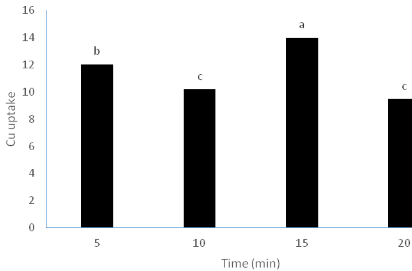
Figure 9. Effect of different time exposure of magnetic field on Cu uptake
