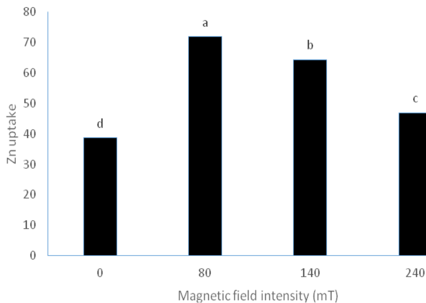
Figure 6. Effect of various magnetic field intensity on plant Zn uptake
