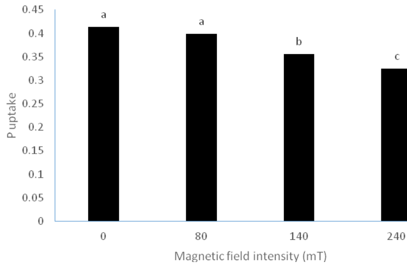
Figure10. Effect of various magnetic field intensity on plant P uptake
