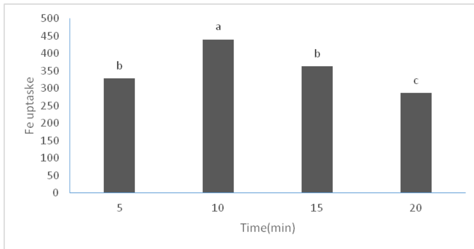
Figure 5. Effect of different time exposure of magnetic field on Fe uptake
