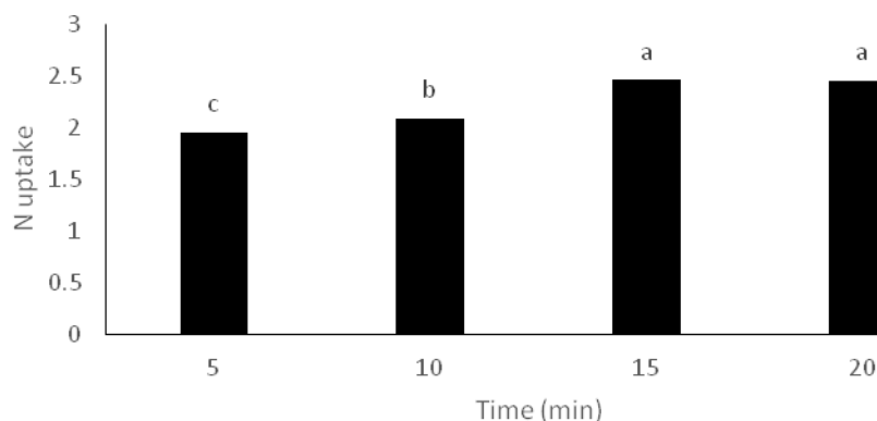
Figure 19. Effect of different time exposure of magnetic field on N uptake
