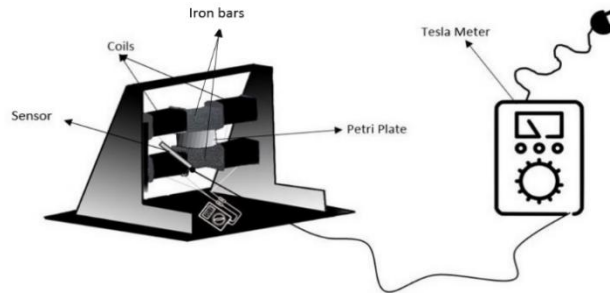
Figure 1. The experimental electromagnet setup (Naz et al. , 2012)
