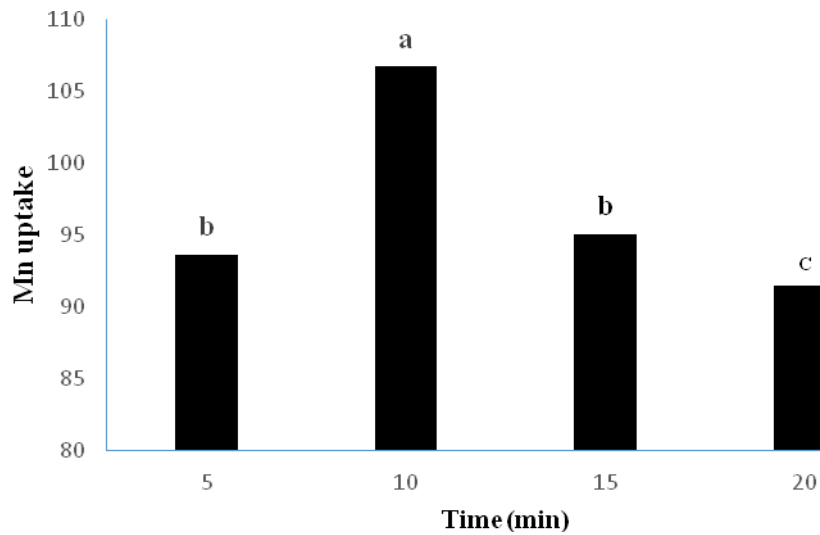
Figure 3. Effect of different time exposure of magnetic field on Mn uptake
