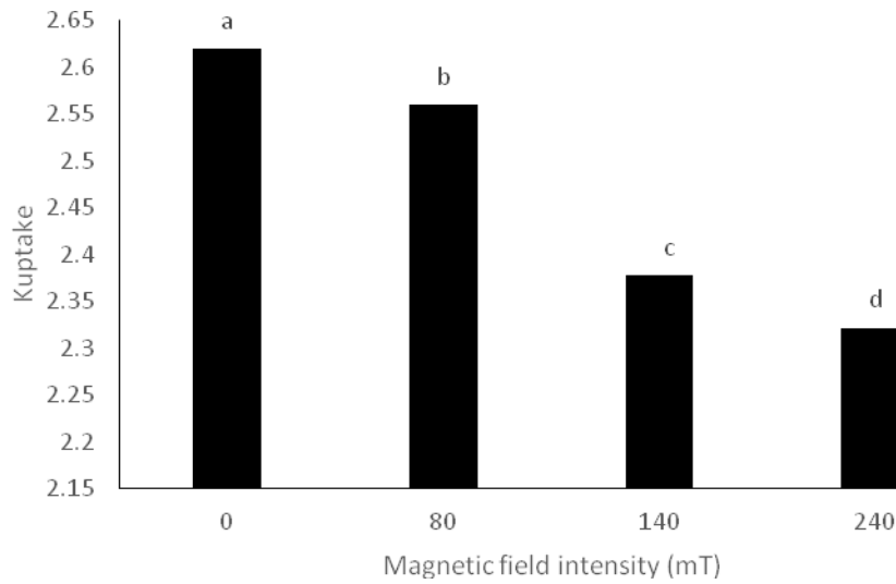
Figure12. Effect of various magnetic field intensity on plant K uptake
