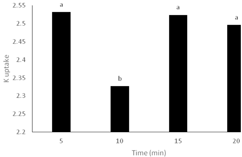
Figure 13. Effect of different time exposure of magnetic field on K uptake
