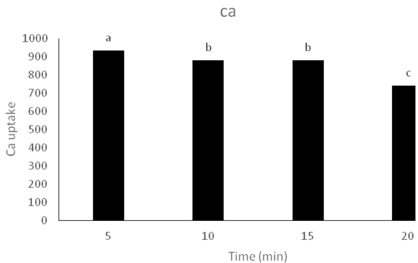
Figure 15. Effect of different time exposure of magnetic field on Ca uptake
