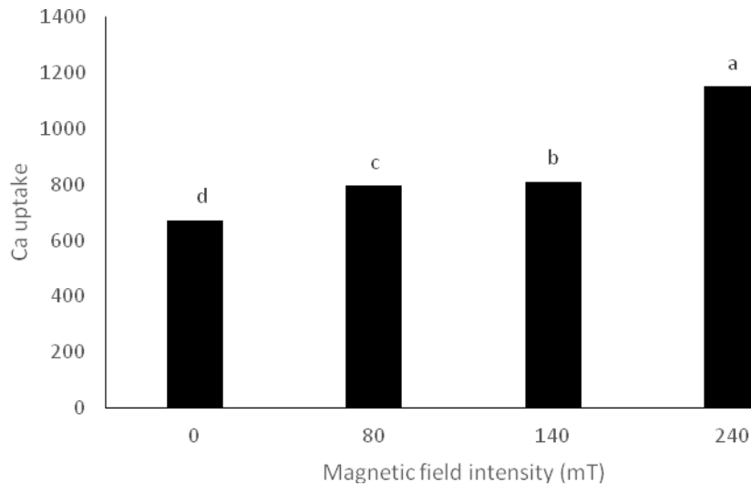
Figure14. Effect of various magnetic field intensity on plant Ca uptake
