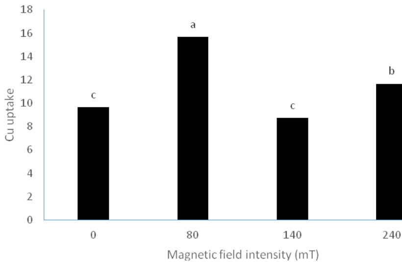
Figure 8. Effect of various magnetic field intensity on plant Cu uptake
