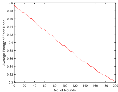
Fig. 5. Average residual energy of sensor nodes
