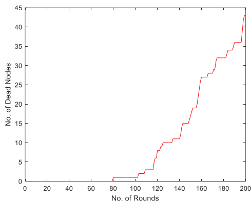
Fig. 6. Death process of the sensor nodes
