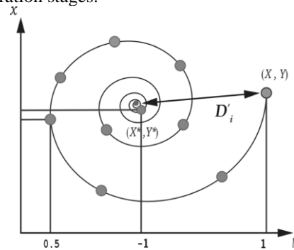
Fig. 2. Spiral updating position
