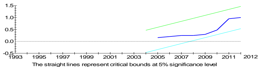
Plot of Cumulative Sum of Squares of Recursive Residuals
