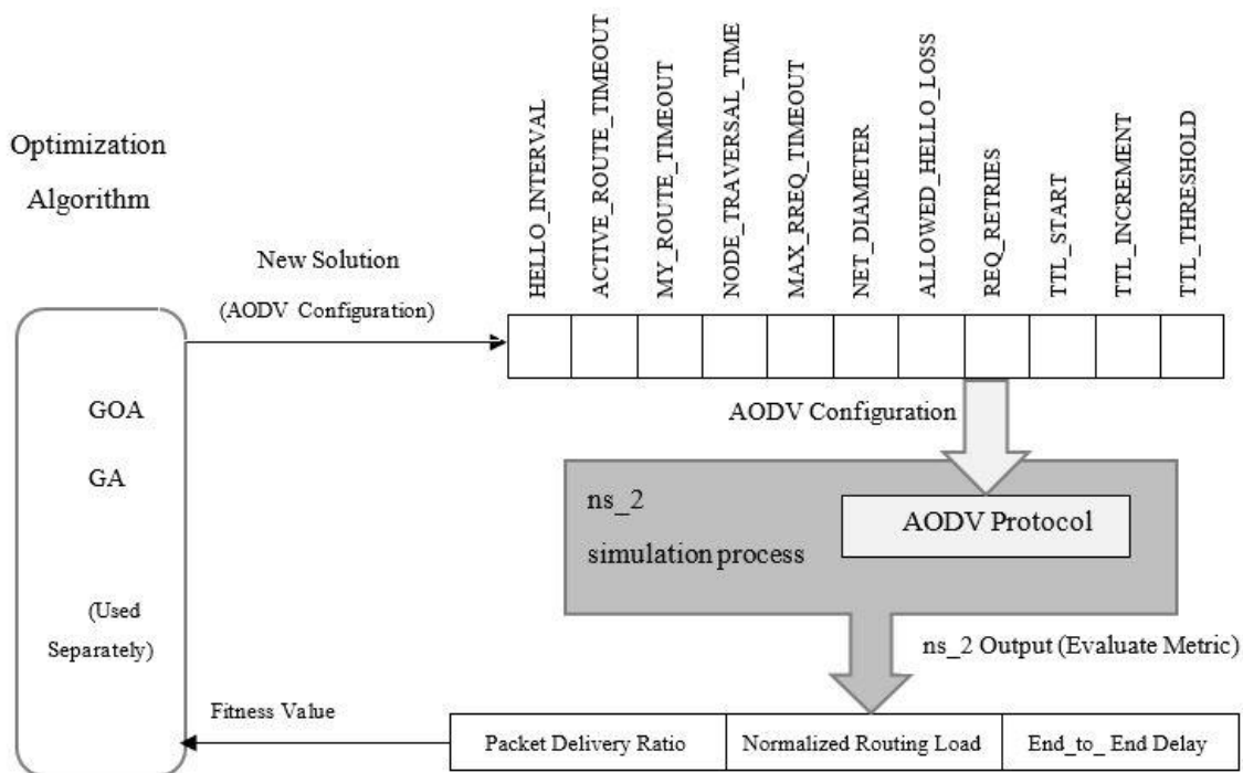
Fig. 1. Optimization framework.
