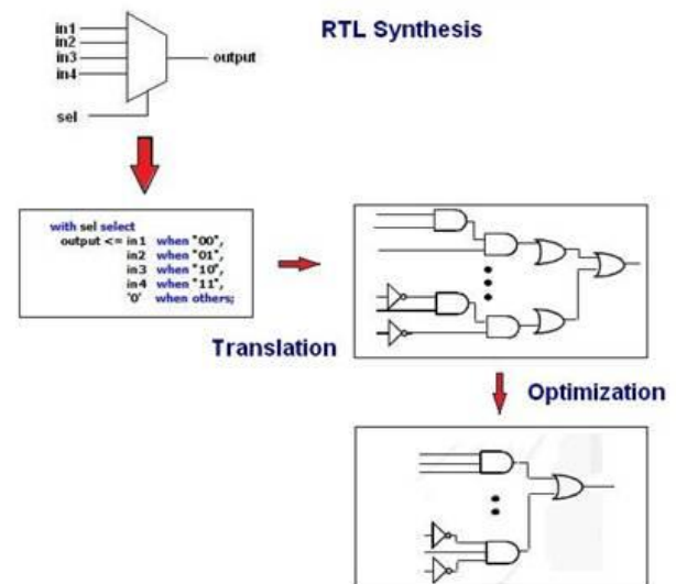
Fig. 1. Software optimization.
