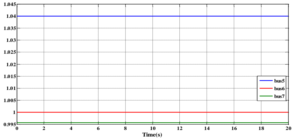
Fig. 17. Voltage of some buses in the presence of DFIG and VPI regulator.
