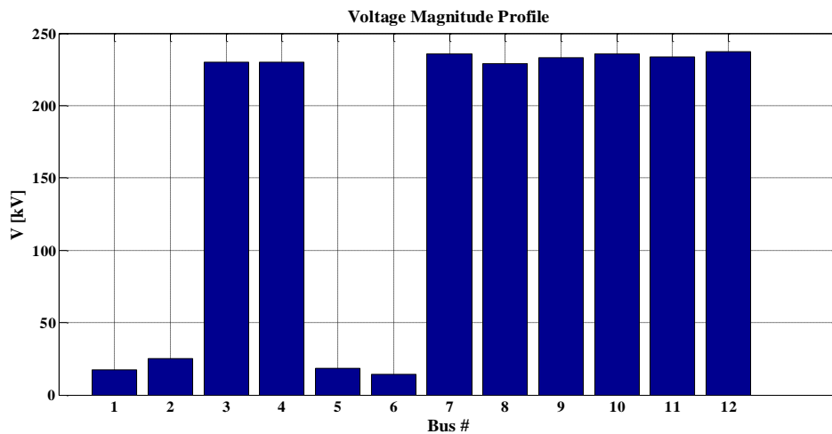
Fig. 18. Bus voltages of the DFIG-based grid and VPI regulator.
