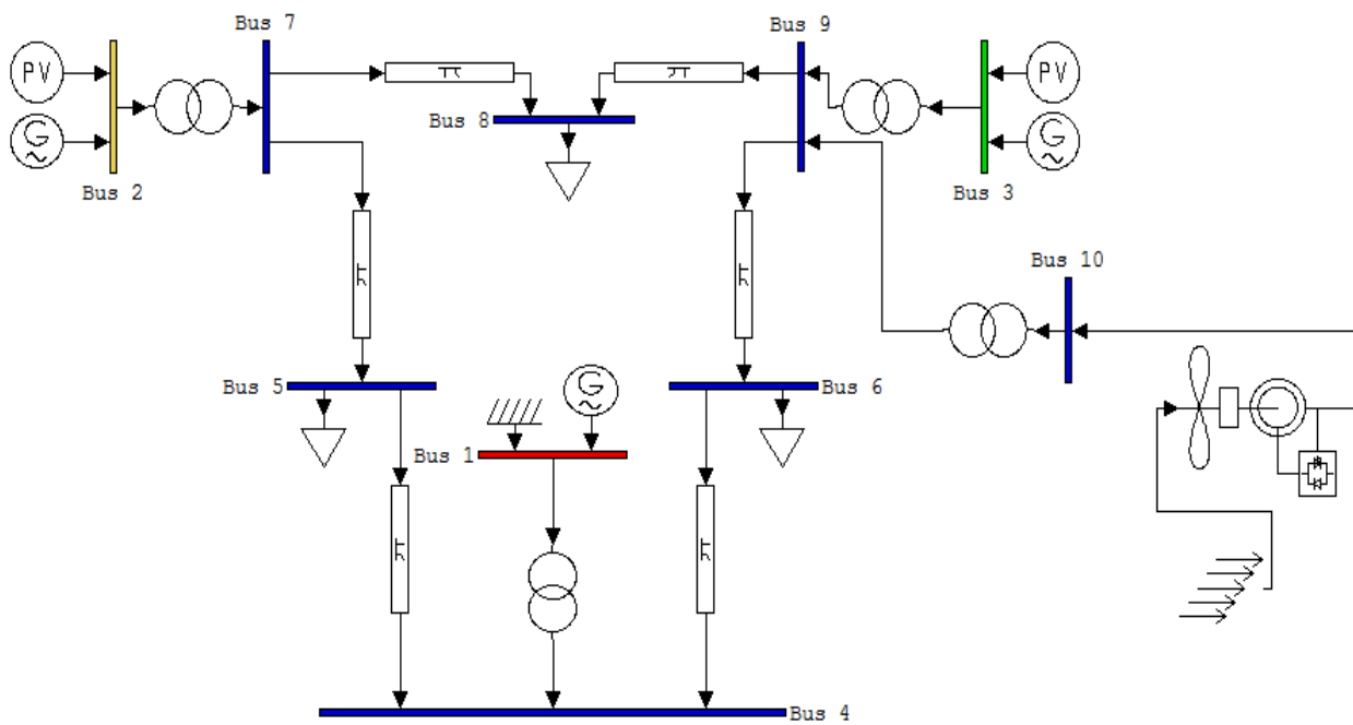
Fig. 13. The studied grid in the presence of DFIG.
