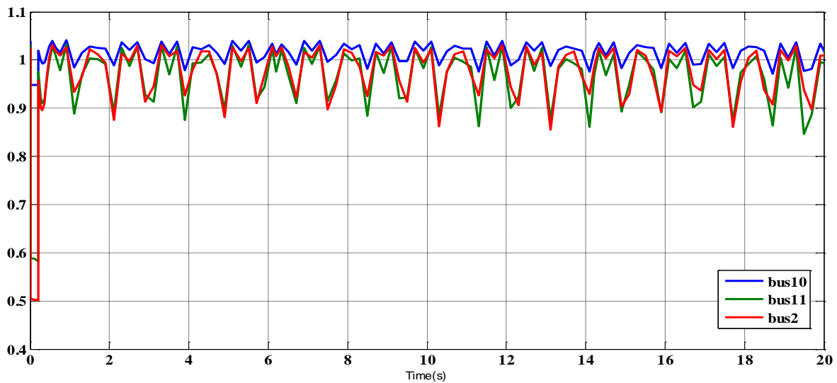
Fig. 14. Voltage of some buses using DFIG.
