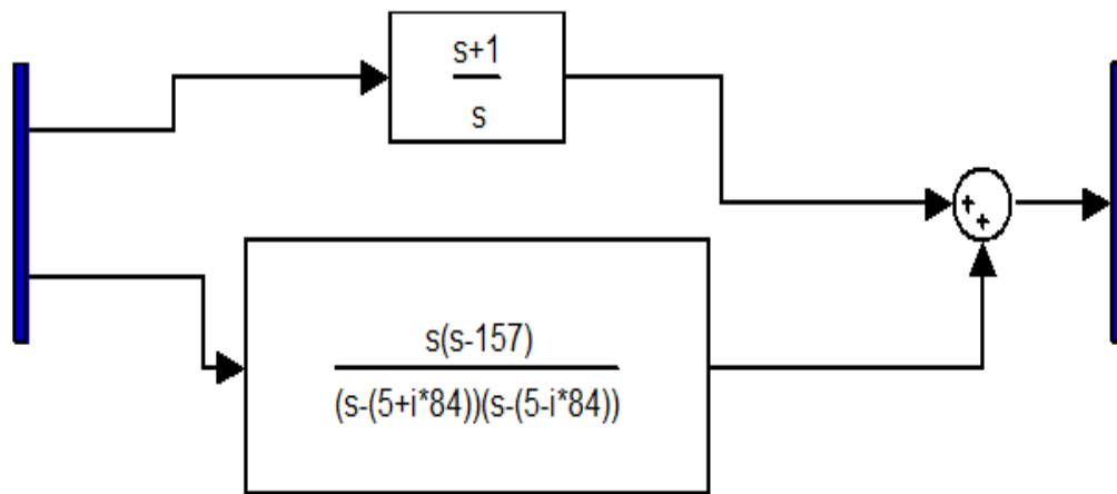
Fig. 1. Block diagram of VPI regulator.
