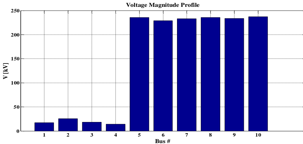
Fig. 15. Bus voltages in the presence of DFIG.
