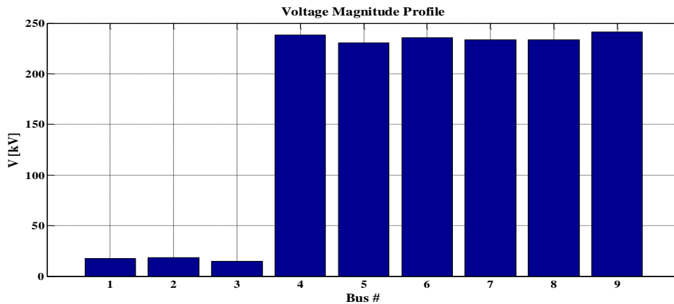
Fig. 12. Voltages of buses in 0.25s fault using SVC compensator.
