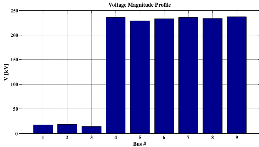
Fig. 6. Voltage of the faultless buses.
