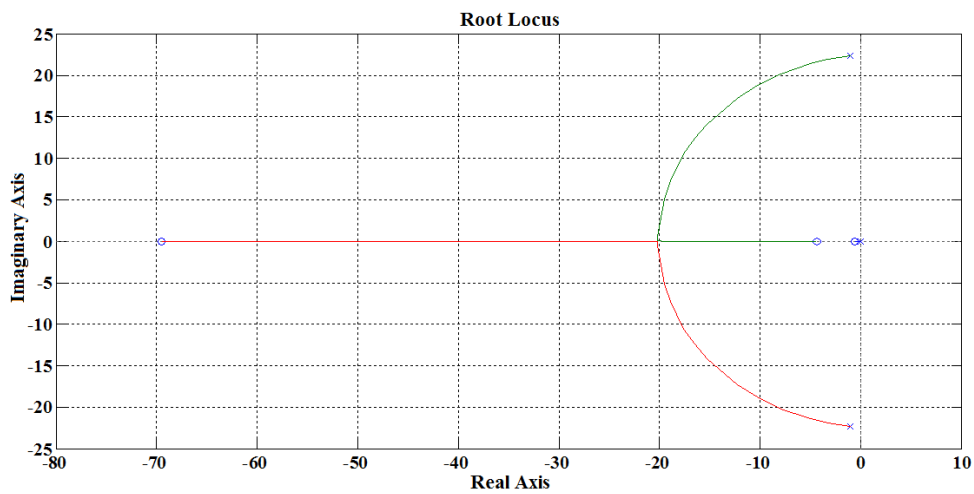
Fig. 3. Closed-loop locus of the VPI poles.
