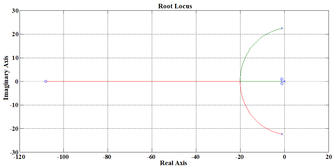
Fig. 2. Open-loop locus of the VPI poles.
