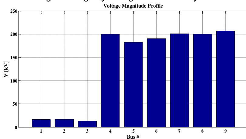
Fig. 8. Voltages of the buses in 0.2s fault
