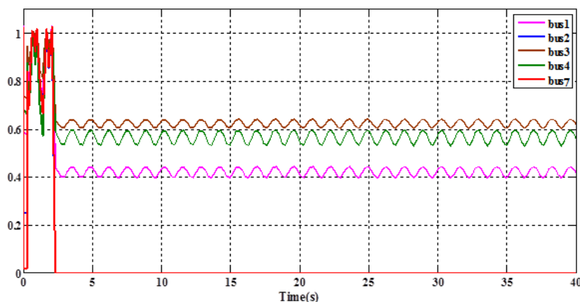
Fig. 9. Voltages of some buses in 0.25s fault.
