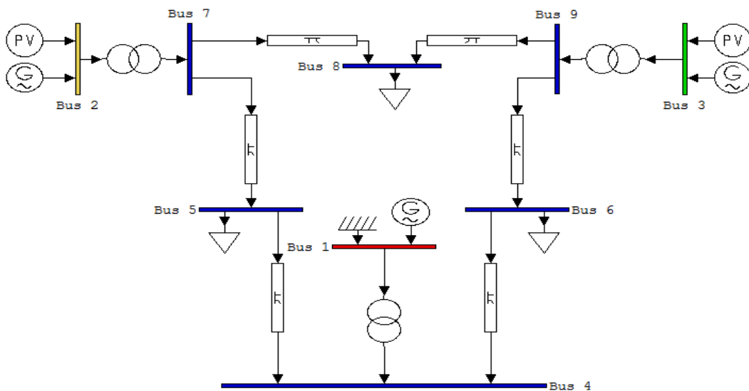
Fig. 4. The studied test network.
