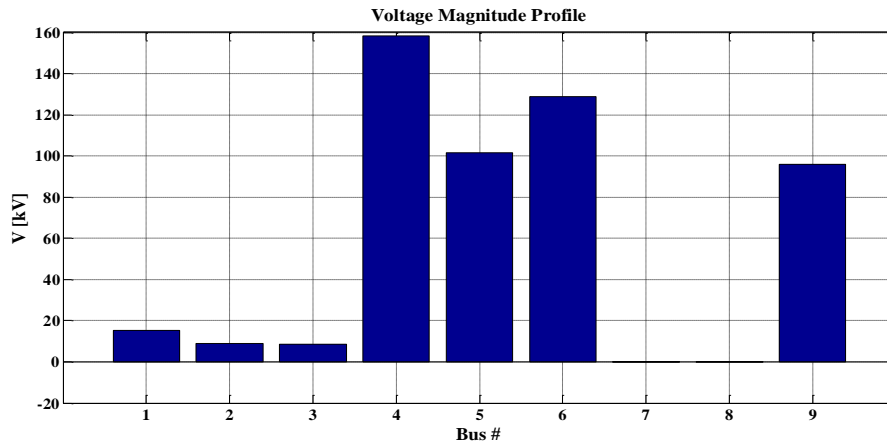
Fig. 10. Voltage of buses in 0.25s fault.
