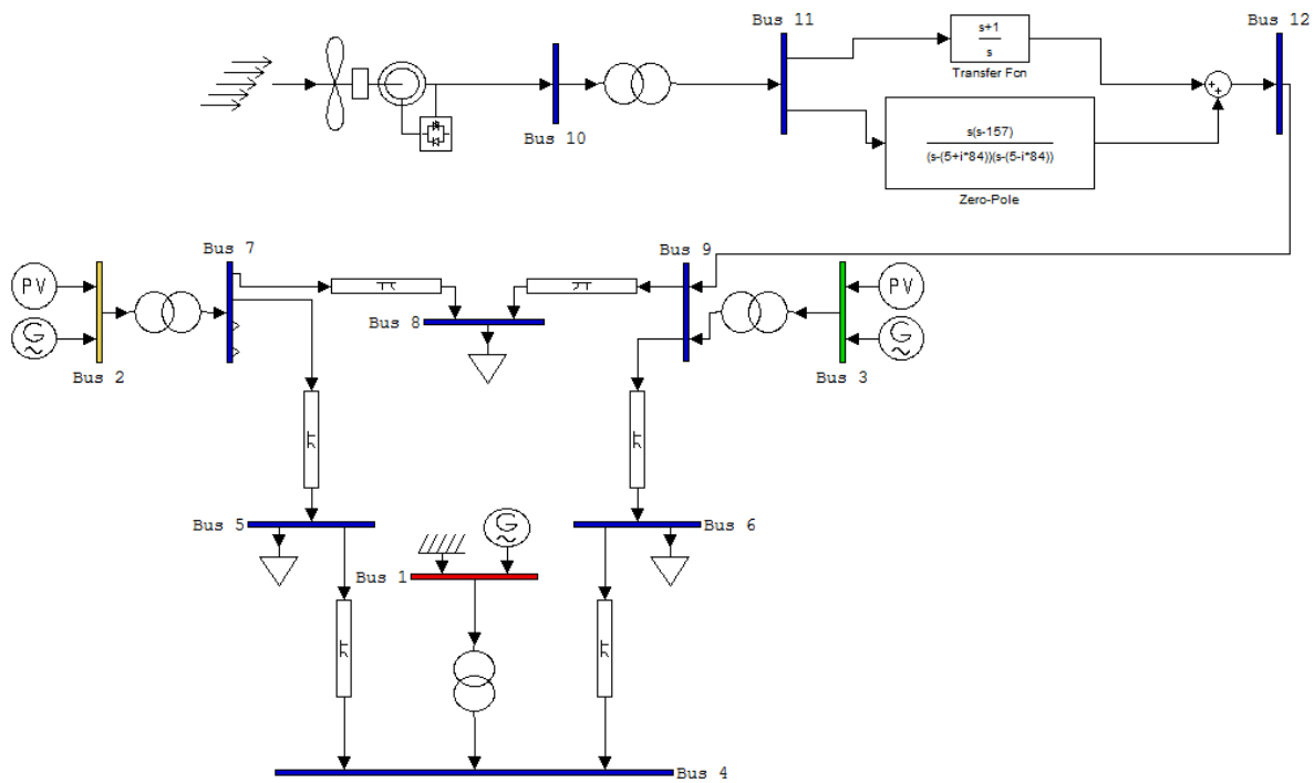
Fig. 16. View of the DFIG-based grid and VPI regulator.
