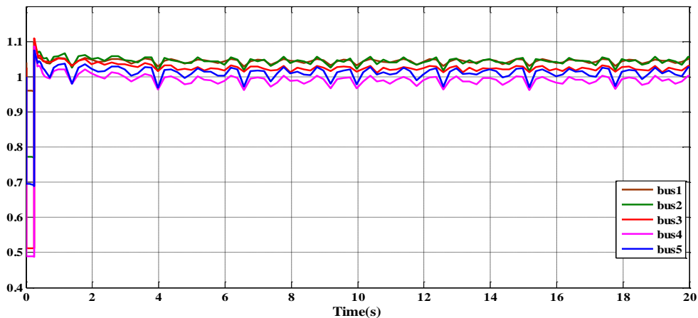
Fig. 11. Voltages of some buses in 0.25s fault using SVC compensator.
