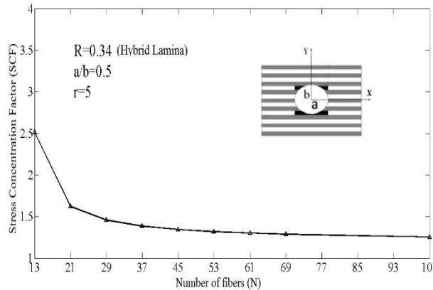
Figure 2) Stress concentration factor as function of different number of fibers (N)
