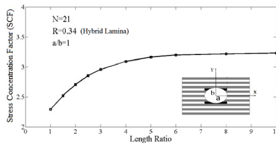
Figure 7) Stress concentration factor as a function of plate length to width ratio
