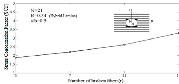
Figure 9) Stress Concentration factor based on the number of broken fibers (HM fibers)
