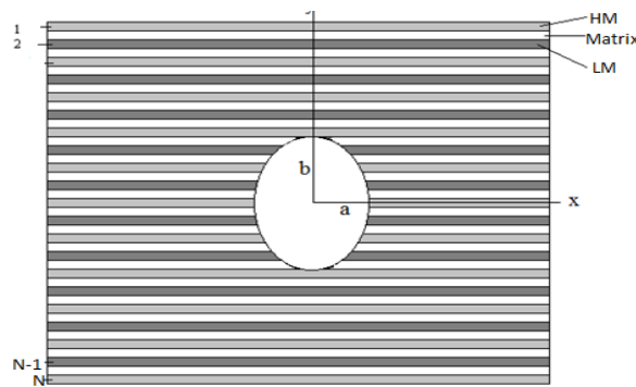
Figure 1) The hybrid plate with elliptical hole in its center under a simple tension stress.
