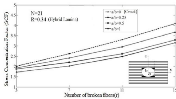
Figure 13) Stress concentration factor in terms of hole ratio
