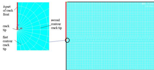
Figure 6) Meshing part of the part and crack tip magnification
