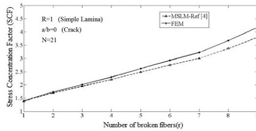
Figure 8) The stress concentration factor comparison FEM and MSLM method
