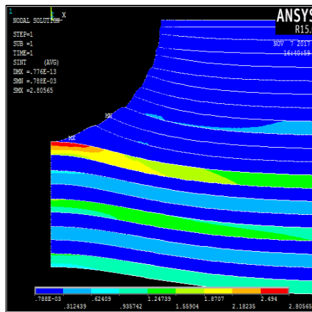
Figure 5) Maximum stress on the plate
