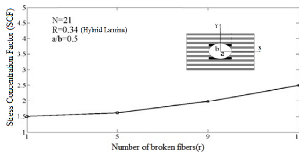
Figure 9) Stress Concentration factor based on the number of broken fibers (HM fibers)
