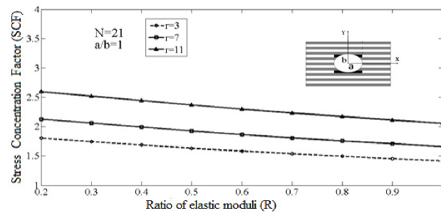
Figure 12) Stress concentration factor as a function of "R" values
