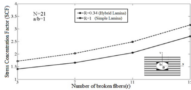
Figure 11) Stress concentration factor in terms of modulus of weak elasticity to strong ratio
