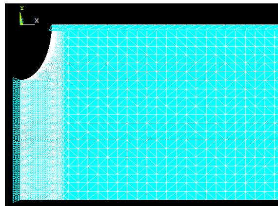
Figure 3) Meshed central part of the hybrid plate
