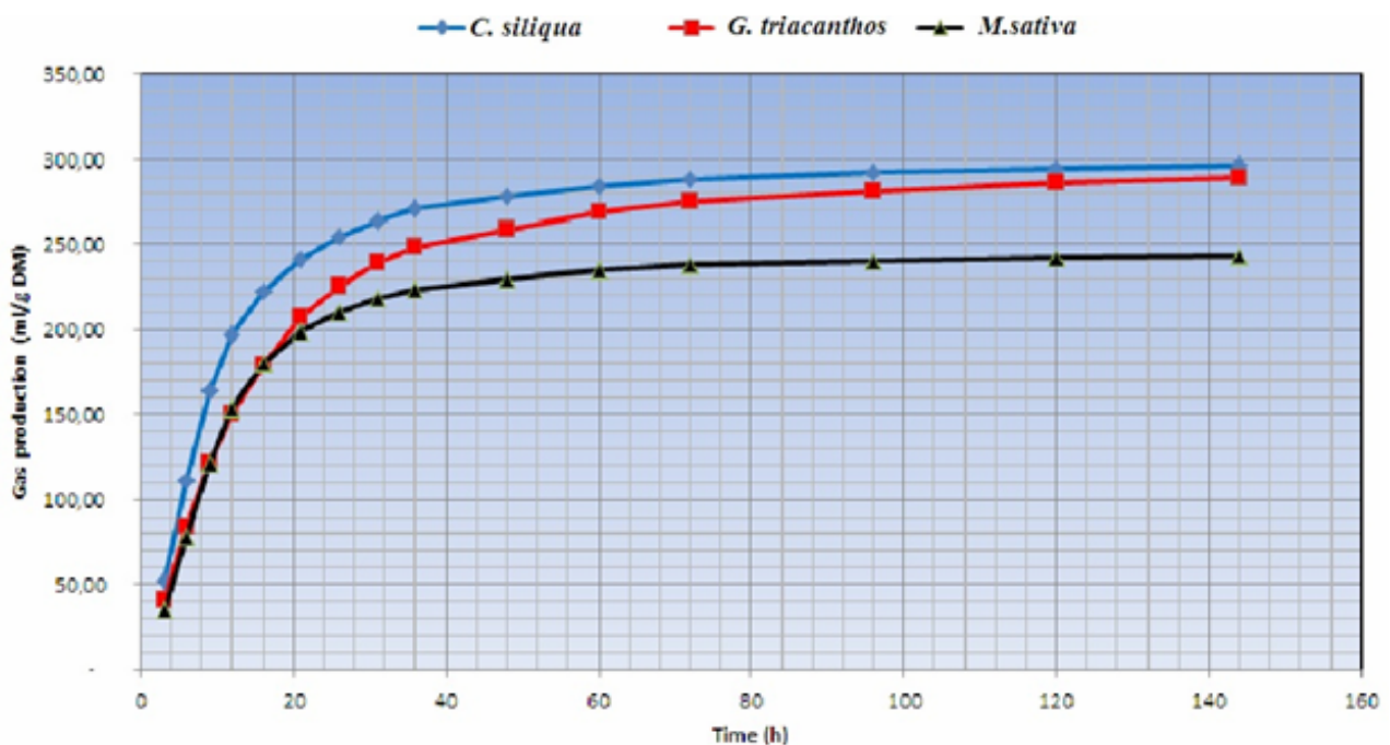
Figure 2 Cumulative gas production profiles
